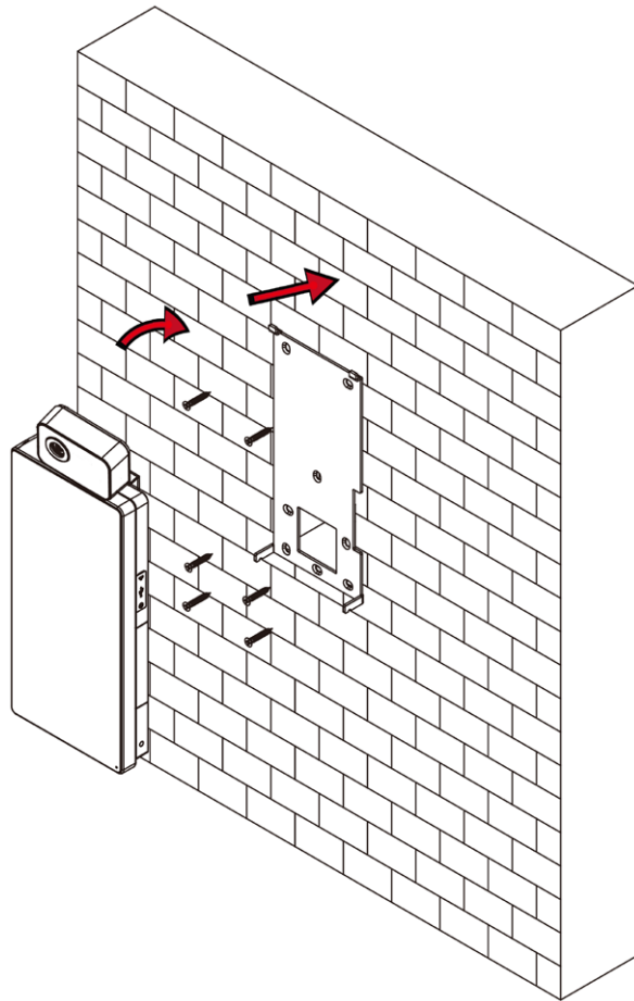
Figure 3-6. Install Device
