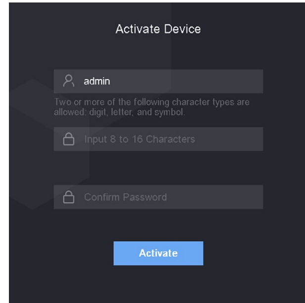
Figure 5-1. Activation Page
