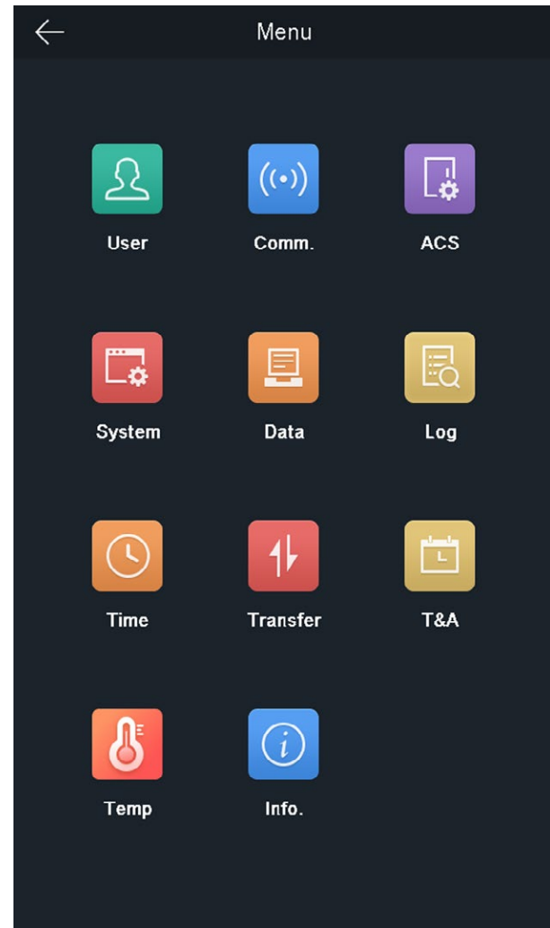
Figure 6-2. Home Page
